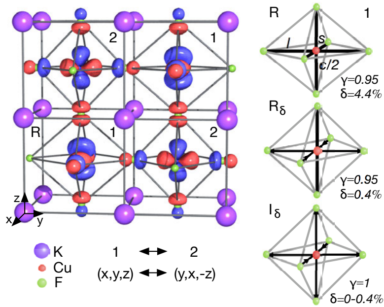
Fig. 1: Crystal structure, distortions, and orbital ordering in \text{KCuF}_3 . Cu is at the center of F octahedra enclosed in a K cage. The conventional cell is tetragonal with axes a , b , c . The pseudocubic axes x , y , z pointing towards neighboring Cu, are shown in the corner. Short ( s ) and long ( l ) CuF bonds alternate between x and y along all pseudocubic axes (co-operative Jahn-Teller distortion). The distortions are measured by \delta=(l-s)/(l+s)/2 and \gamma=c/a\sqrt{2} . R is the experimental structure ( \gamma=0.95 , \delta=4.4\% ), R_\delta ( \gamma=0.95 ) and I_\delta ( \gamma=1 ) two ideal structures with reduced distortions. In the I_0 structure the cubic crystal-field at the Cu site splits the 3d manifold into a t_{2g} triplet and a e_g doublet. In the R structure, site symmetry is lowered further by the tetragonal compression ( \gamma<1 ) and the Jahn-Teller distortion ( \delta \neq 0 ). The figure shows the highest-energy 3d orbital. From Ref. [3].
