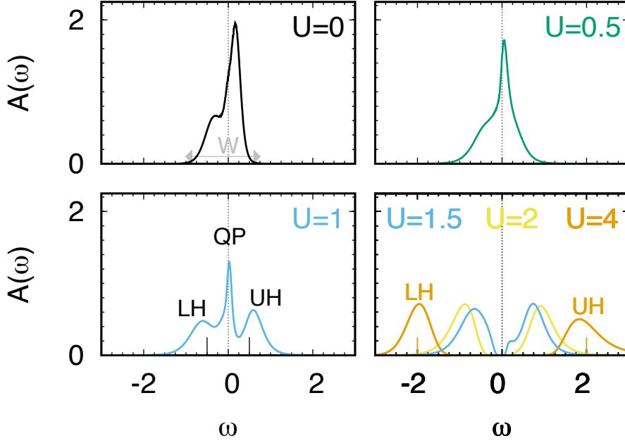
Fig. 8: \text{VOMoO}_4 : LDA+DMFT spectral function at finite temperature for 0 \leq U \leq 4 . Energies are in eV and spectral functions in states/spin/eV. The calculations have been done using a continuous-time hybridization-expansion QMC solver [13]. A detailed LDA+DMFT study of the electronic and magnetic properties of \text{VOMoO}_4 can be found in Ref. [15].
